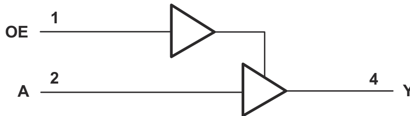
Figure 8-1. Logic Diagram
