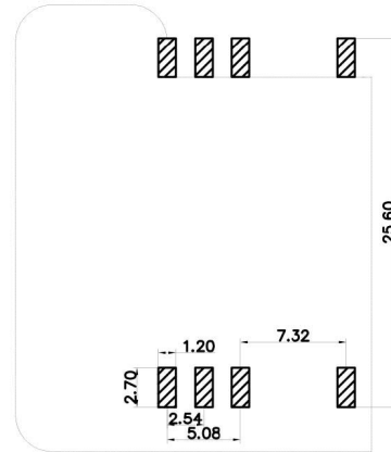
RECOMMEND P. C. BOARD LAYOUT
