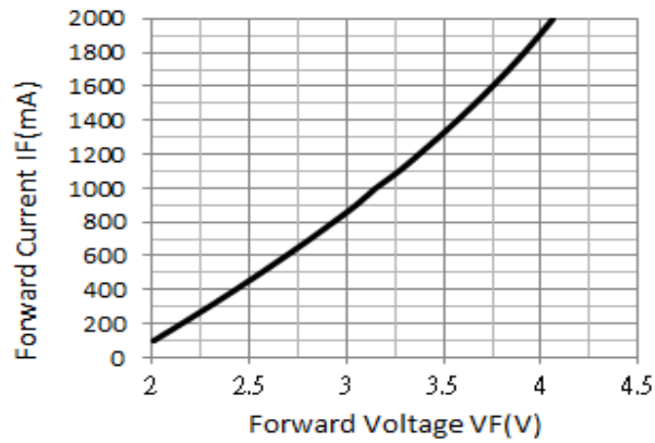
Fig 4. Forward Current
