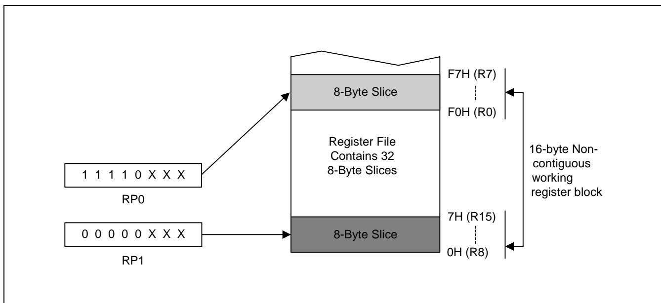
Figure 2-10. Non-Contiguous 16-Byte Working Register Block
