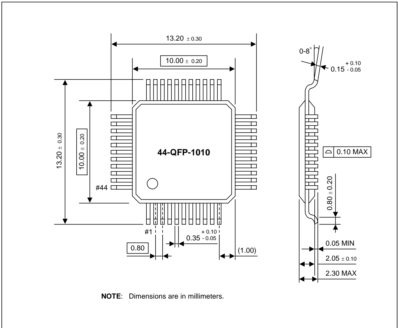
Figure 22-2. 44-QFP-1010 Package Dimensions
