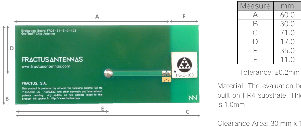
Figure 1 – EB_FR05-S1-E-0-103. Geofind™ Evaluation Board.
