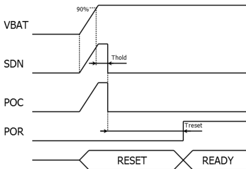
Figure 7. Start-up phase
