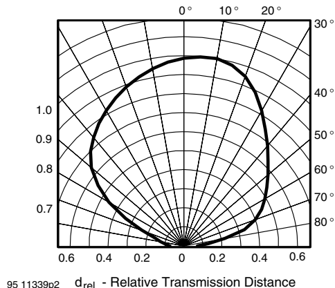
Fig. 12 - Vertical Directivity
