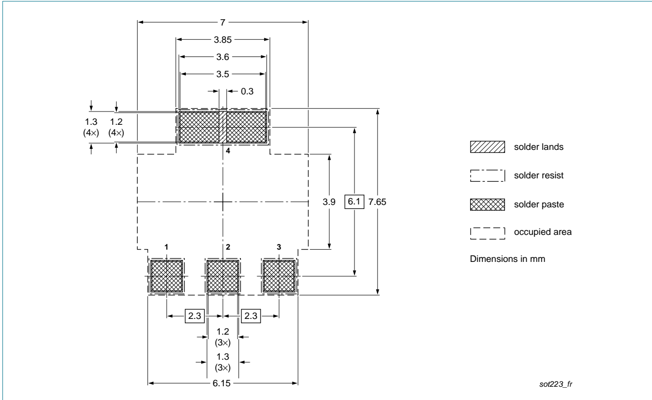
Fig 19. Reflow soldering footprint SOT223 (SC-73)
