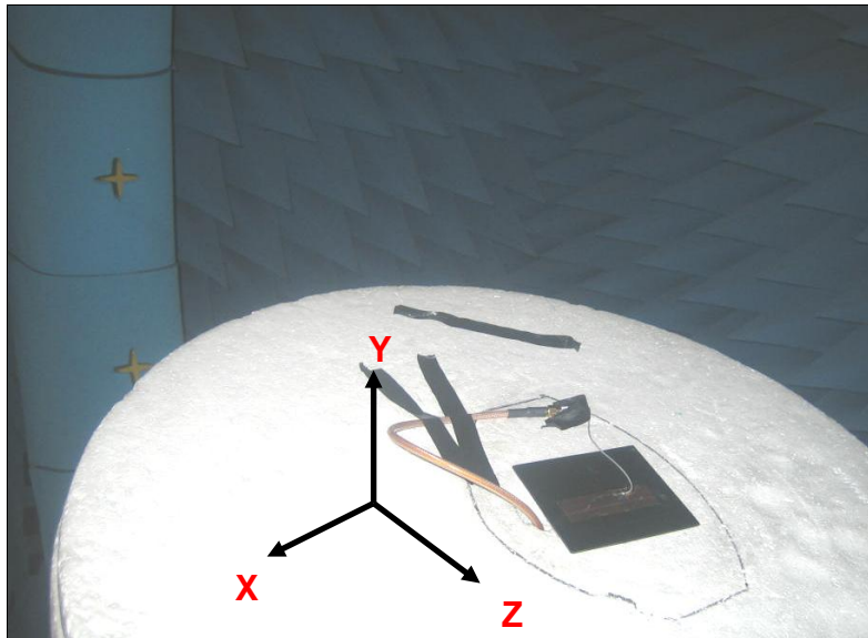
Figure 1. Satimo System.
