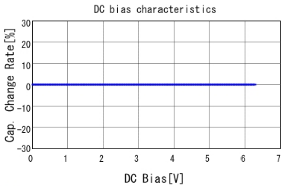
■ GJM0335C0J220JB01 C-DC bias capchange, 25.0degC, AC1V
