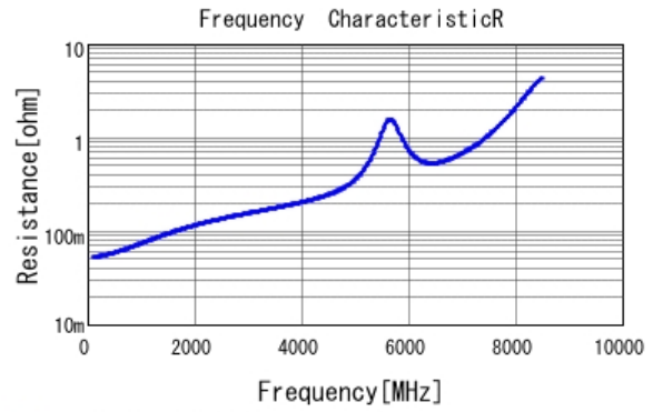
■ GJM0335C0J220JB01 R DC0V, 25degC
