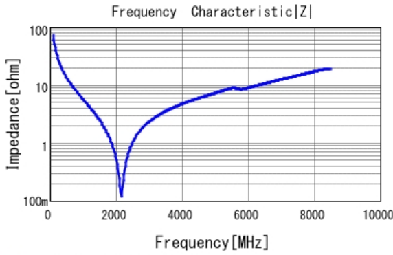
■ GJM0335C0J220JB01 |Z| DC0V, 25degC
