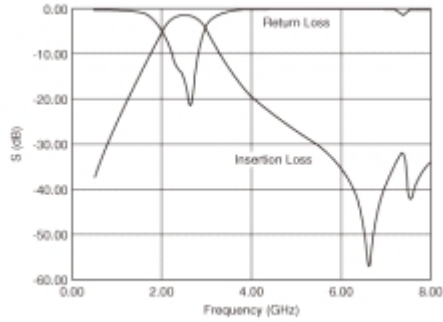
Frequency Characteristics
