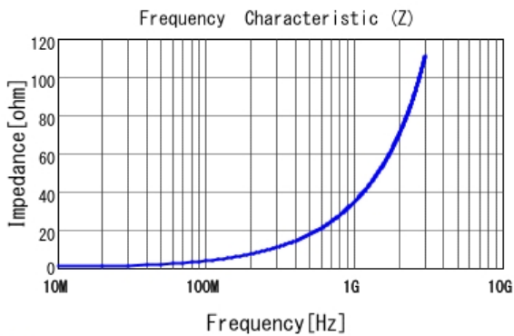
■ LQP02TN5N6J02 |Z|
