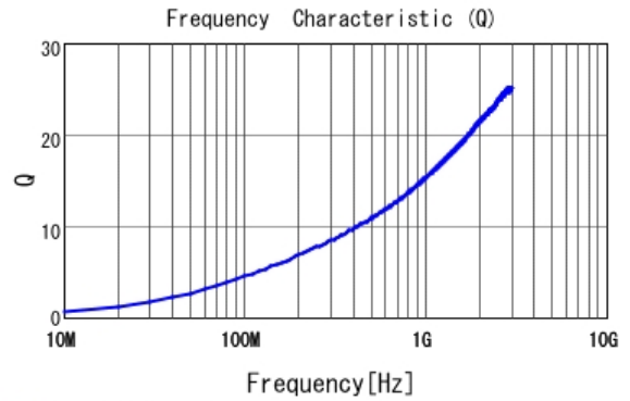
■ LQP02TN5N6J02 Q
