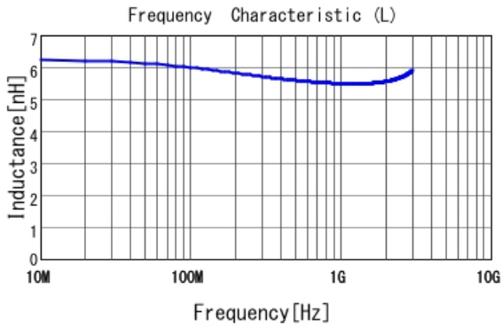
■ LQP02TN5N6J02 L
